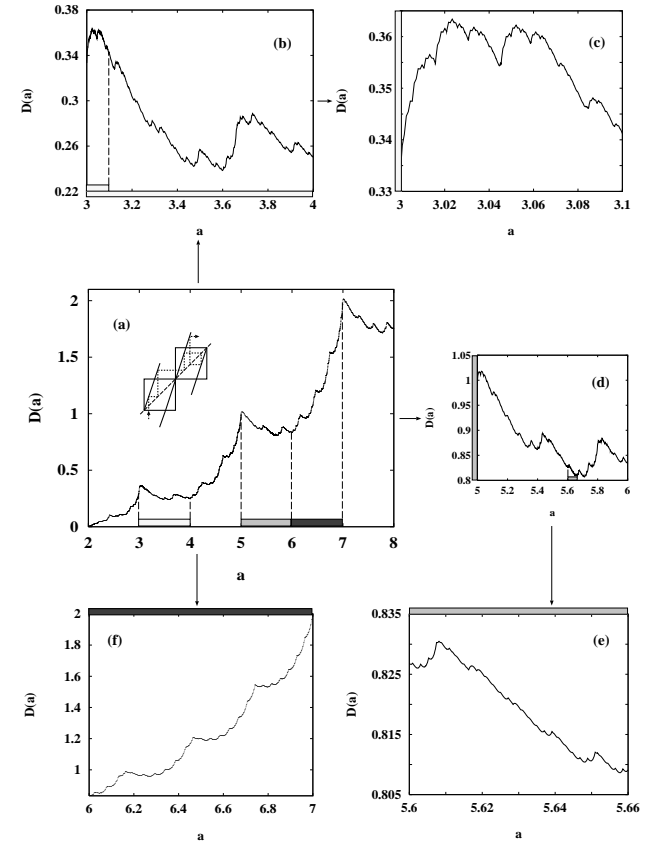
Figure 24.5: The dependence of D on the map parameter a is continuous, but not monotone. Here a stands for the slope \Lambda in (24.9). (From ref. [24.9].)
