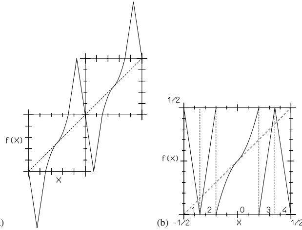
Figure 24.6: (a) A map with marginal fixed point. (b) The map restricted to the unit circle.
