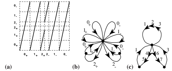
Figure 24.4: (a) A partition of the unit interval into six intervals, labeled by the jumping number \hat{n}(x) \in \{0_+, 1_+, 2_+, 2_-, 1_-, 0_-\} . The partition is Markov, as the critical point is mapped onto the right border of M_{1_+} . (b) The transition graph for this partition. (c) The transition graph in the compact notation of (24.26) (introduced by Vadim Moroz).
