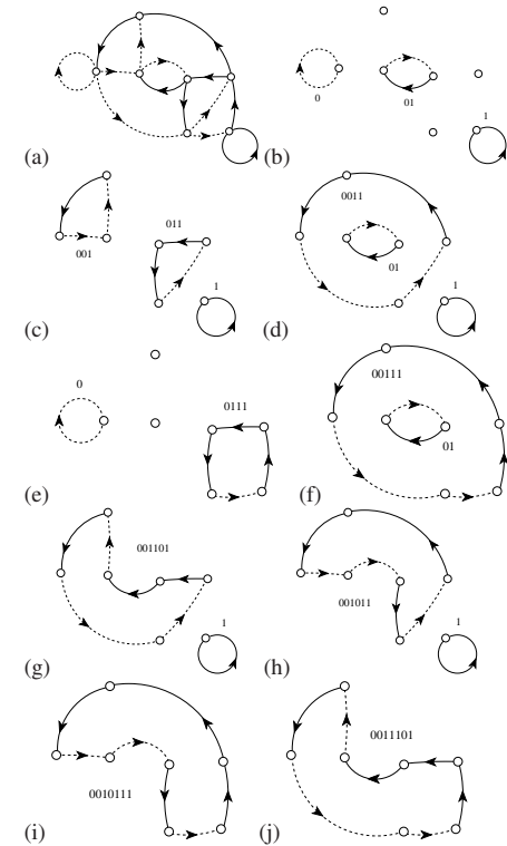
Figure 18.3: (a) The region labels in the nodes of transition graph figure 17.4 can be omitted, as the links alone keep track of the symbolic dynamics. (b)-(j) The fundamental cycles (18.35) for the transition graph (a), i.e., the set of its non-self-intersecting loops. Each loop represents a local trace t_p , as in (17.5).
