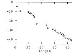
Figure 18.1: The logarithm \ln|z_0^{(n)} - z_0| of the difference between the leading zero of the n -th polynomial approximation to topological zeta function and our best estimate (18.23), as a function of order of the polynomial n (the topological zeta function evaluated for the closest value of A to A = 3.8 for which the quadratic map has a stable cycle of period n ). (from K.T. Hansen [15.23])
