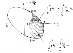
Figure 36.3: S_p(E) , the action of a periodic orbit p at energy E , equals the area in the phase space traced out by the 1-dof trajectory.
