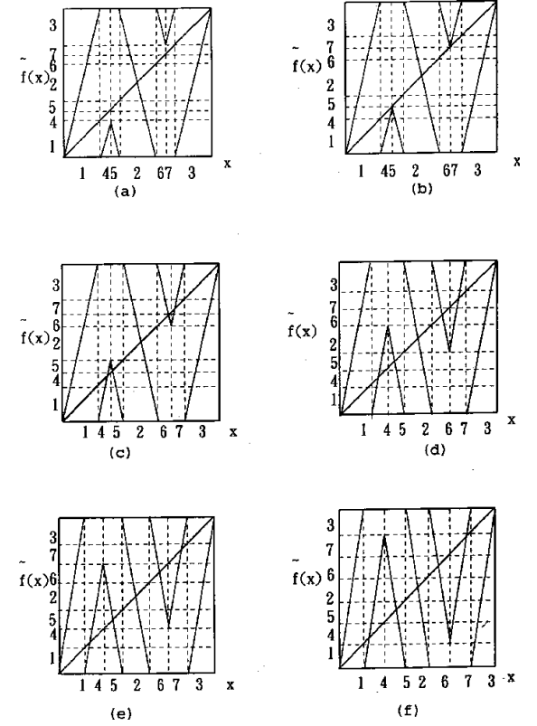
Figure T.1: (a)-(f) The sawtooth map (T.1) for the 6 values of parameter a for which the folding point of the map aligns with the endpoint of one of the 7 intervals and yields a finite Markov partition (from ref. [T.1]). The corresponding transition graphs are given in figure T.2.
