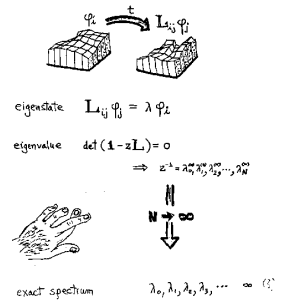
Figure 16.4: State space discretization approach to computing averages.
