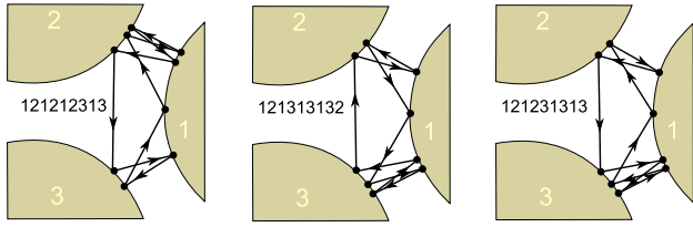
Figure 9.7: Cycle \overline{121212313} has multiplicity 6; shown here is \overline{121313132} = \sigma_{23}\overline{121212313} . However, \overline{121231313} which has the same stability and period is related to \overline{121313132} by time reversal, but not by any C_{3v} symmetry.
