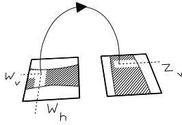
Figure 23.4: For an analytic hyperbolic map, specifying the contracting coordinate w_h at the initial rectangle and the expanding coordinate z_v at the image rectangle defines a unique trajectory between the two rectangles. In particular, w_v and z_h (not shown) are uniquely specified.
