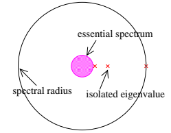
Figure 23.5: Spectrum of the Perron-Frobenius operator acting on the space of \mathbb{C}^{k+\alpha} Hölder-continuous functions: only k isolated eigenvalues remain between the spectral radius, and the essential spectral radius which bounds the “essential,” continuous spectrum.
